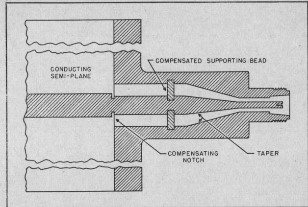
Figure 3. Cross Section of Basic Transition Section
