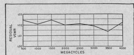
Figure 4. Residual VSWR of Typical 805A Slotted Line
